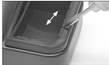
Use the slots to remove remaining particles.
